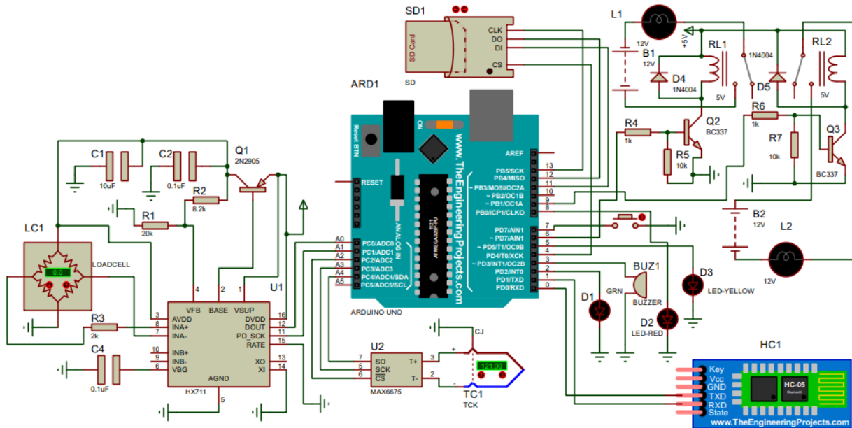
Figure 10: Circuit Design
